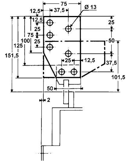
Spreader for connection to cables with lugs
